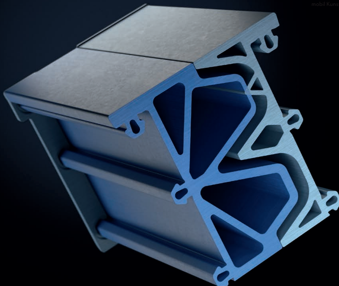
Reworked profiles
